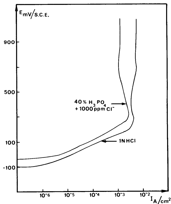
FIGURE 1 — Anodic behavior of pure tungsten.
