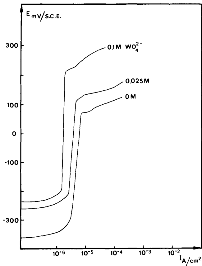
FIGURE 2 — Anodic behavior of 16Cr-14Ni steels in 0.1 M NaCl with various \text{WO}_4^{2-} additions.
