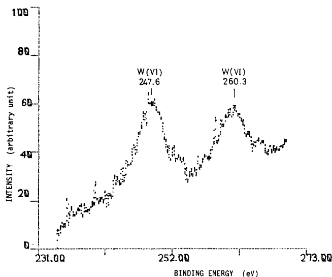
FIGURE 4 — ESCA spectrum of 16Cr-14Ni steel passivated in 0.1 M NaCl + 0.05 M \text{WO}_4^{2-} .
